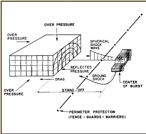
Fig. 3 – Blast loading on buildings.
