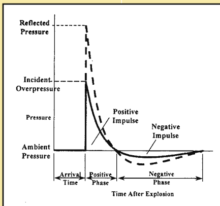
Fig. 2 – Qualitative pressure-time history. SOURCE: “Structures to Resist the Effects of Accidental Explosions,” TM5-1300, November, 1990.
