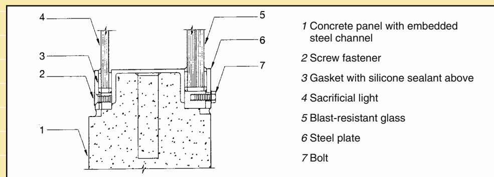
Fig. 15 – Blast-resistant glazing detail.
