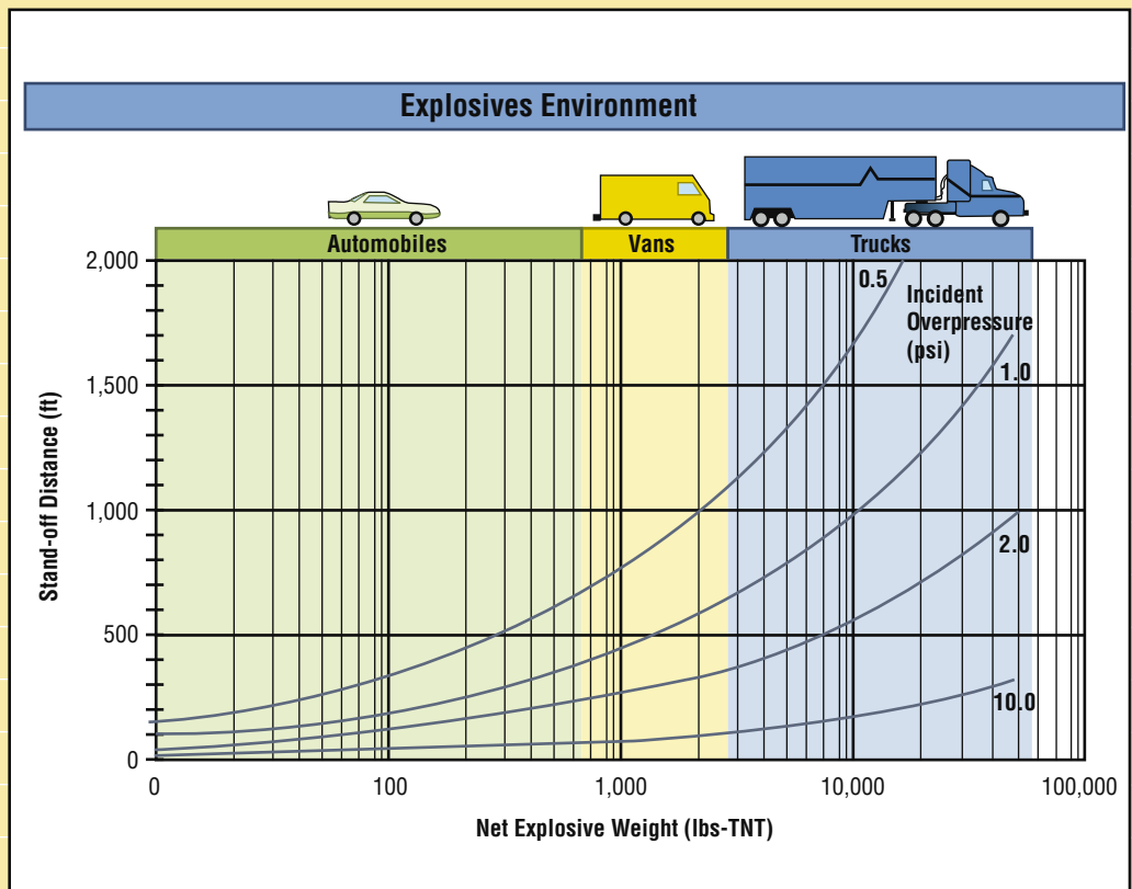
Fig. 4 – Incident overpressure measured in pounds per square inch, as a function of stand-off distance and net explosive weight (pounds-TNT). Source: Federal Emergency Management Agency, Reference Manual to Mitigate Potential Terrorist Attacks, FEMA 426 (Washington, DC: Federal Emergency Management Agency, December 2003).
