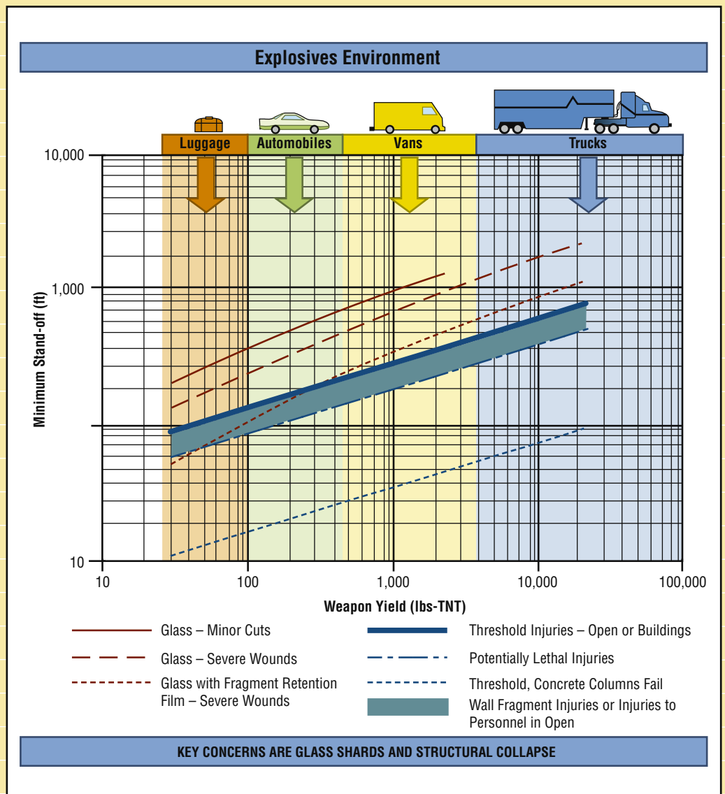
Fig. 5 – Explosives environments – blast range to effects. Source: Federal Emergency Management Agency. Reference Manual to Mitigate Potential Terrorist Attacks. FEMA 426 (Washington, DC: Federal Emergency Management Agency, December 2003).
