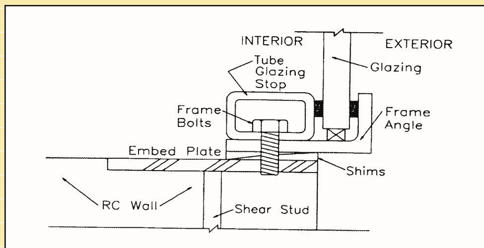
Fig. 14 – Generic blast window glazing and frame detail. Source: Structural Design for Physical Security: State of the Practice, Structural Engineering Institute of American Society of Civil Engineers, Reston, VA, 1999.
