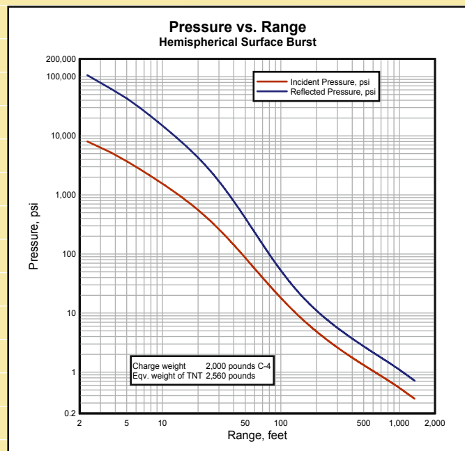
Fig. 6 – Pressure vs. Range-Hemispherical Surface Burst.* *Bridge and Tunnel Vulnerability Workshop, U.S. Army Engineer Research and Development Center, Vicksburg, MS, May 13-15, 2003
