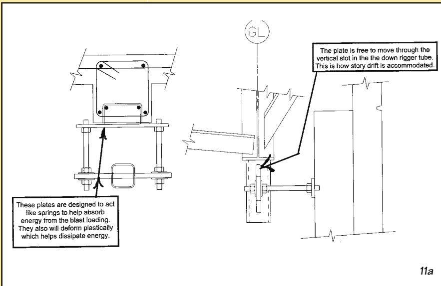
Fig. 11a through 11b – Push/pull or tie-back connections
