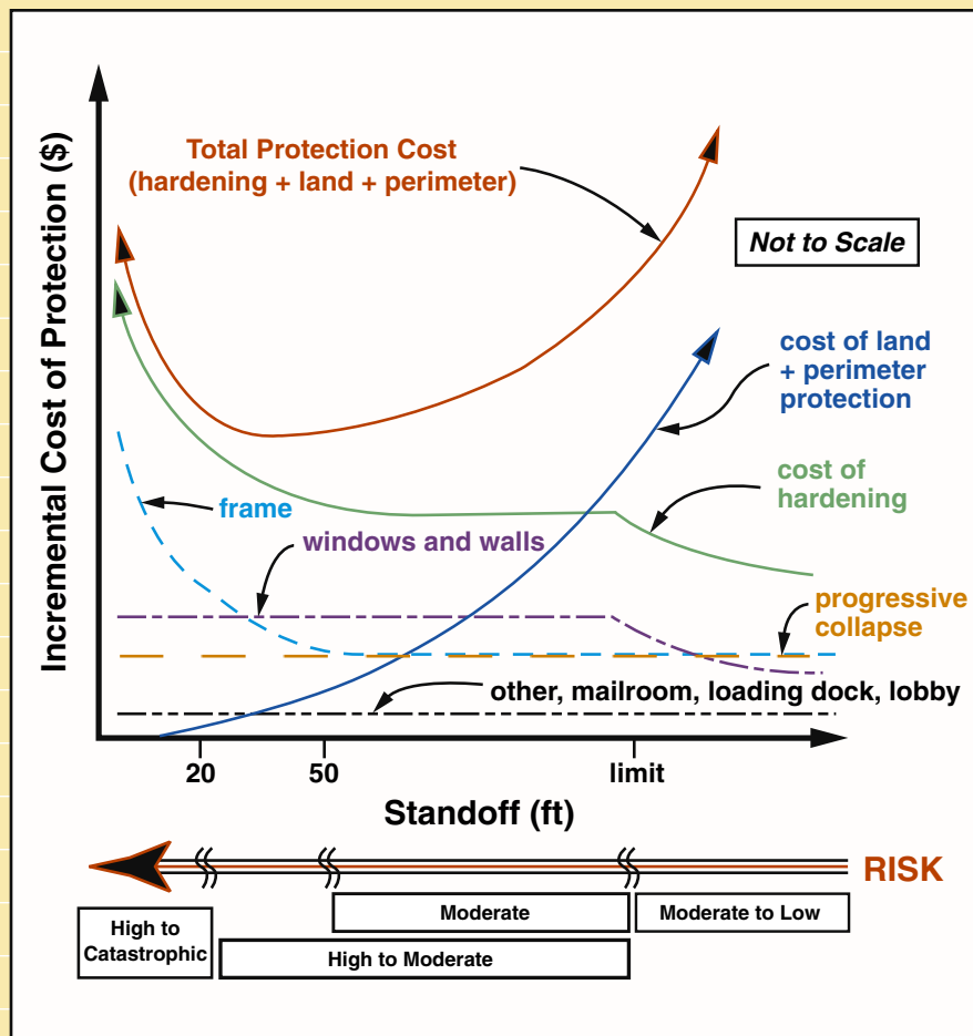
Fig. 16 – Plots showing relationship between cost of upgrading various building components, standoff distance, and risk. Source: Federal Emergency Management Agency. Primer for Design of Commercial Buildings to Mitigate Terrorist Attacks . FEMA 427 (Washington, DC: Federal Emergency Management Agency, December 2003).
