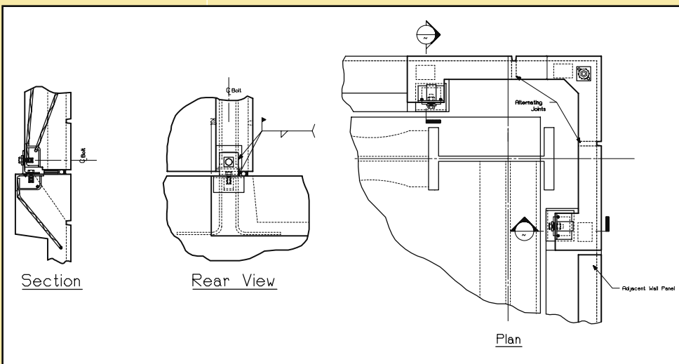
Fig. 12 – Column cover connection
