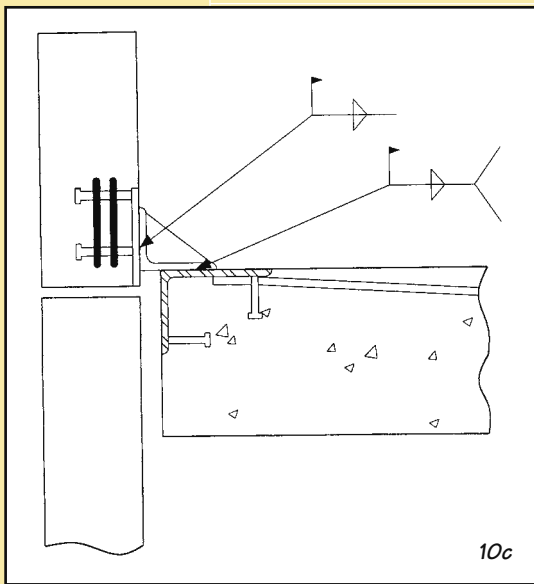
Fig. 10a through 10f - Bearing connections
