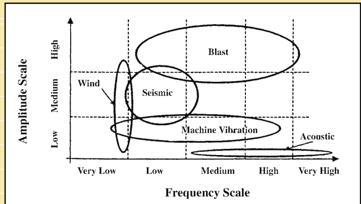
Fig. 1 – Qualitative amplitude-frequency distribution for different hazards. SOURCE: Ettouney, M., "Is Seismic Design Adequate for Blast?" Society of American Military Engineers National Symposium on Comprehensive Force Protection, Charleston, S.C., November 2001.
