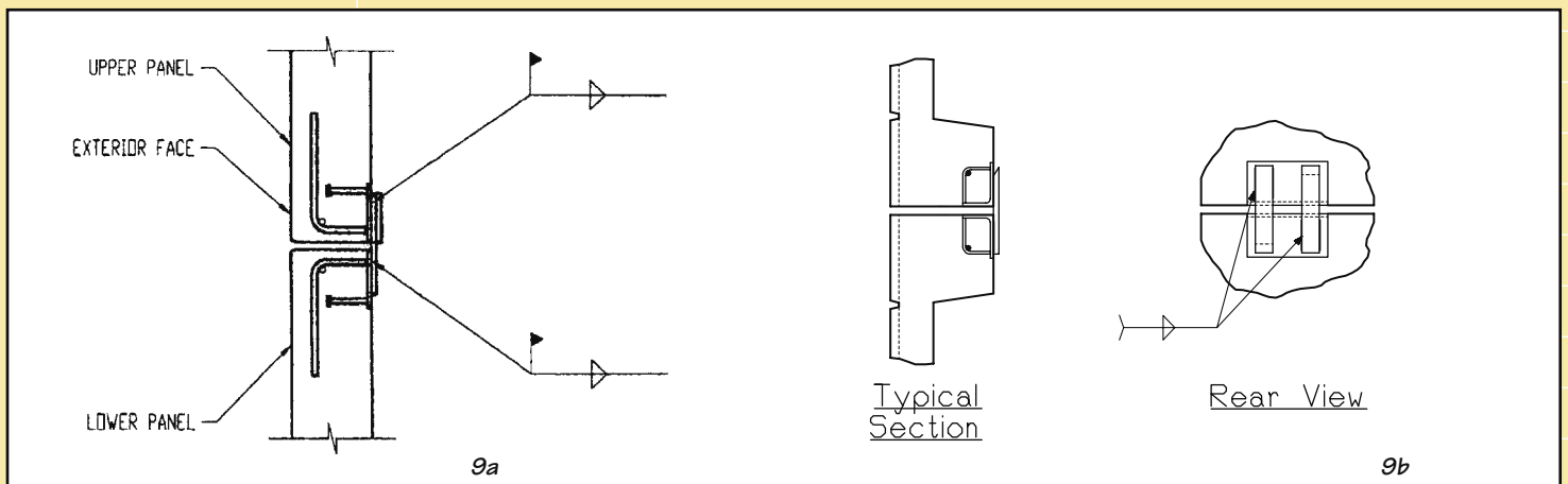
Fig. 9a through 9b – Panel to panel or alignment connections
